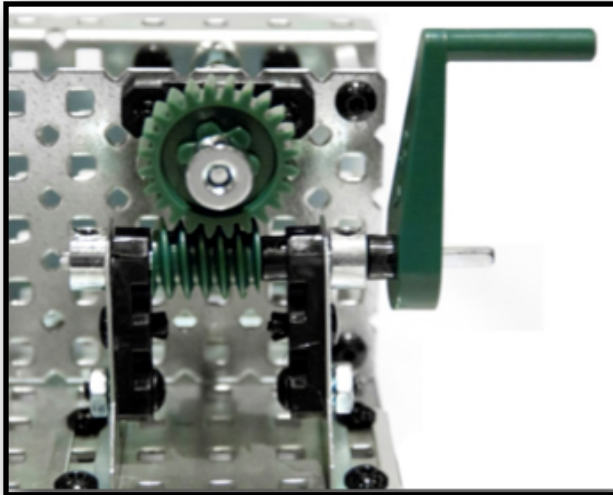
Worm and Wheel
